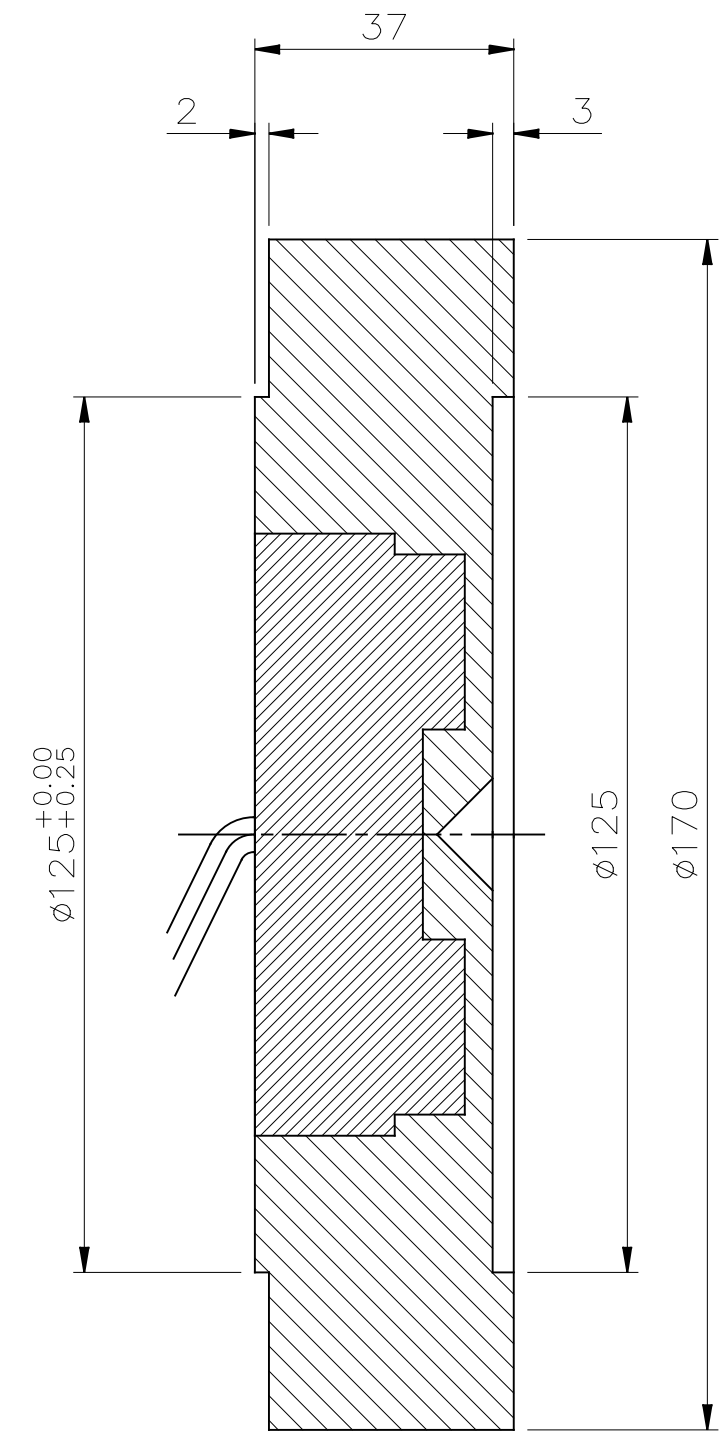
SECTION AA
