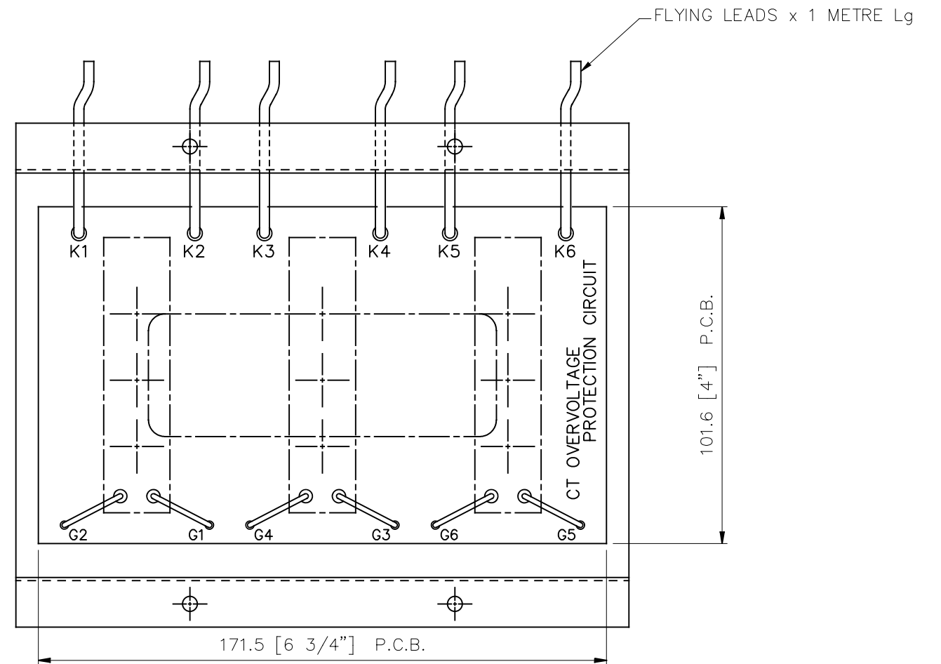
VIEW ON ARROW 'X'
